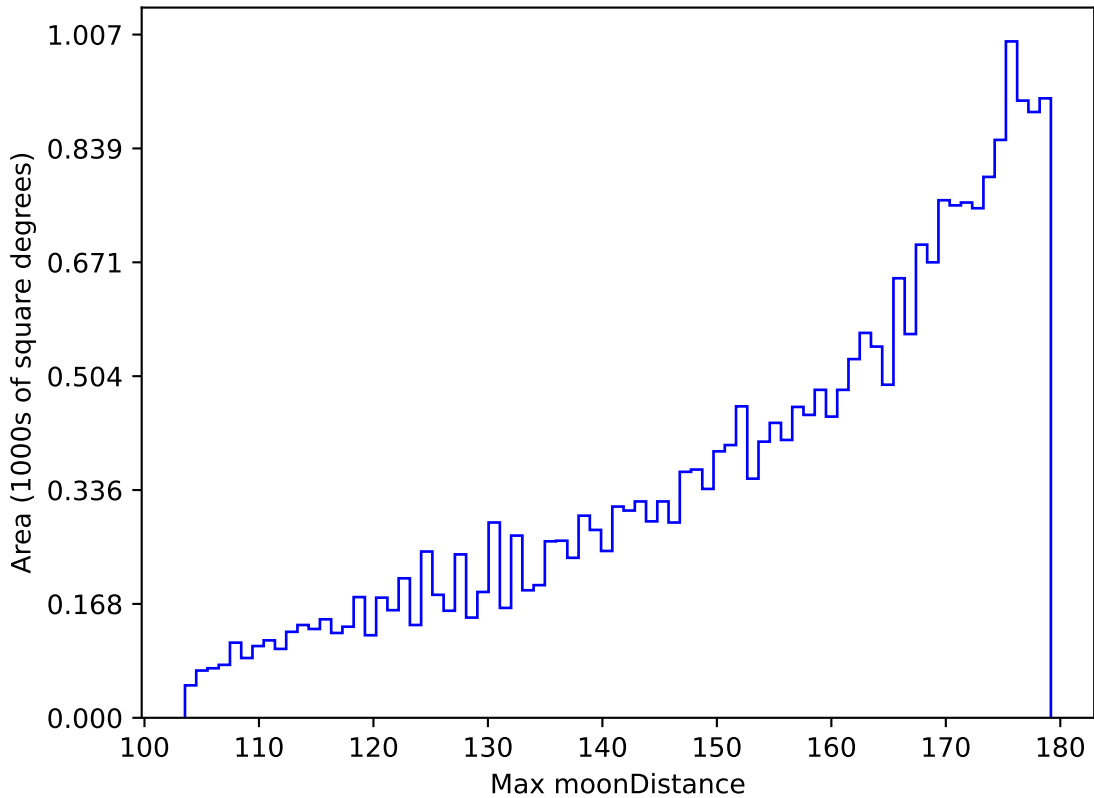
too_elab_r32_d2_ugrizy_v3.4_10yrs All sky i band: Max moonDistance
