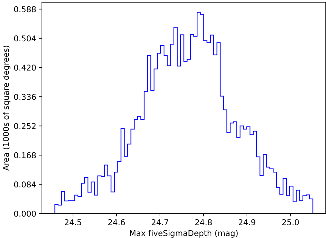
too_elab_r32_d2_ugrizy_v3.4_10yrs WFD r band: Max fiveSigmaDepth
