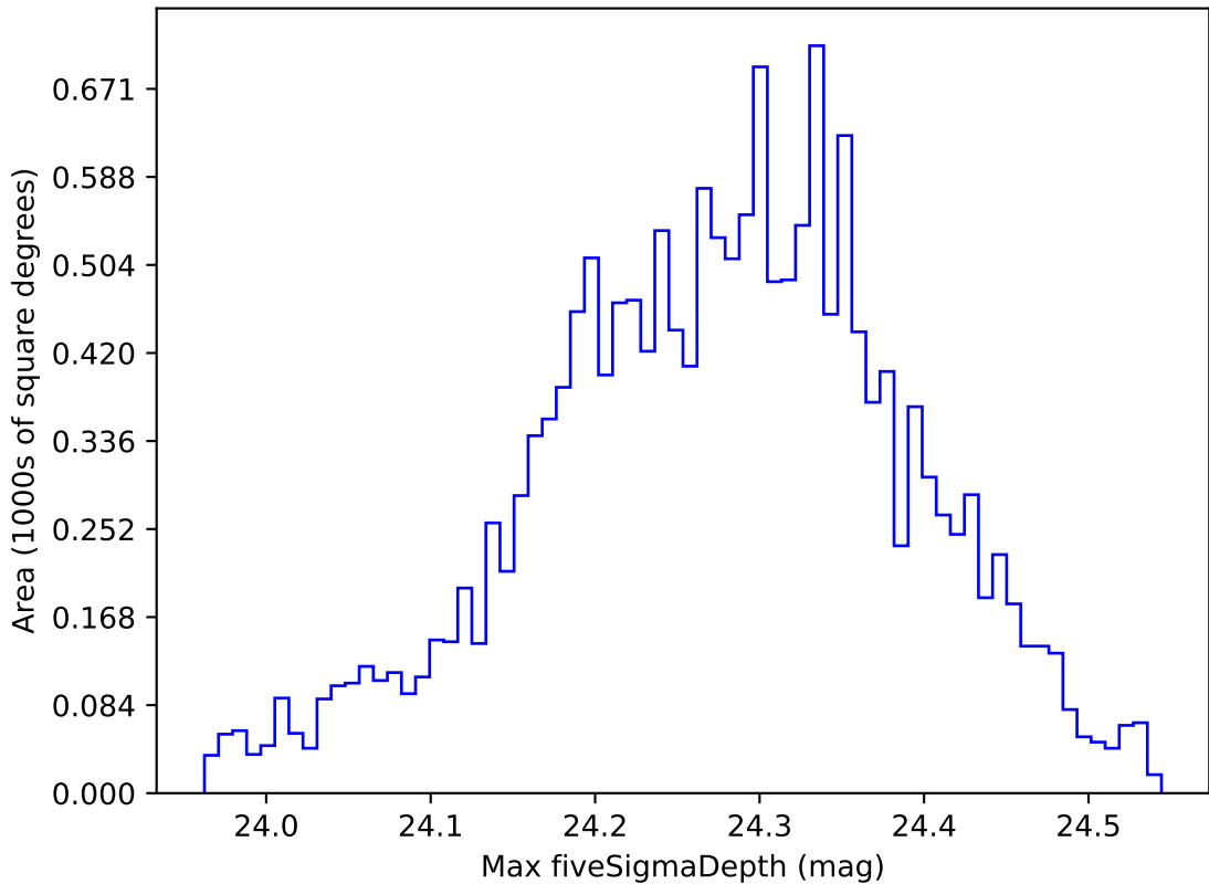
too_elab_r32_d2_ugrizy_v3.4_10yrs WFD i band: Max fiveSigmaDepth
