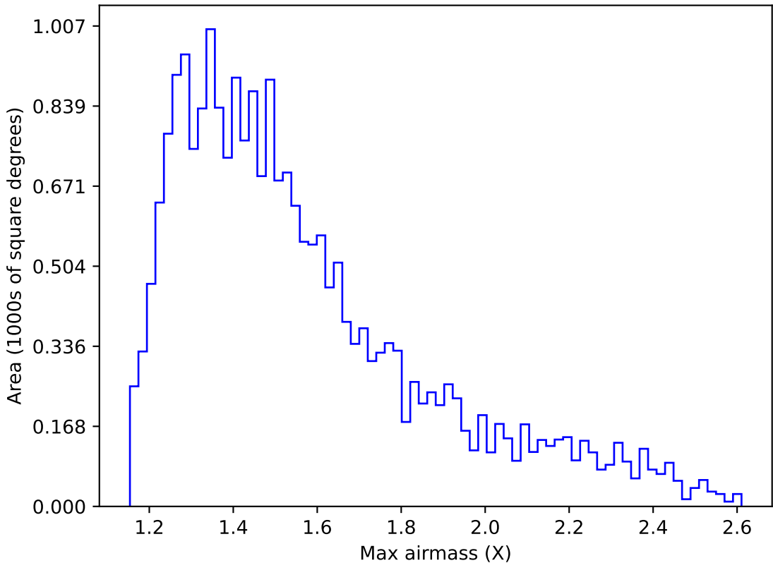
too_elab_r32_d2_ugrizy_v3.4_10yrs Yr 1 y band: Max airmass
