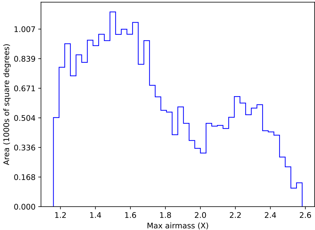
too_elab_r32_d2_ugrizy_v3.4_10yrs Yr 1 r band: Max airmass
