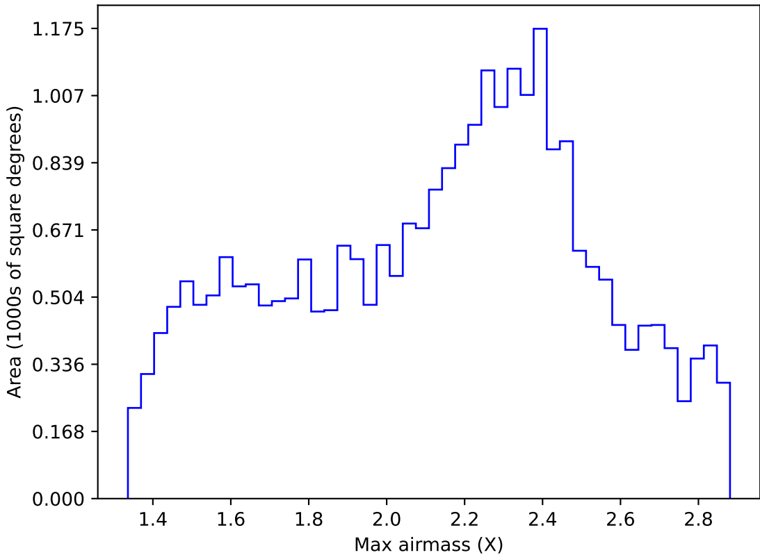
too_elab_r32_d2_ugrizy_v3.4_10yrs Yr 1 all bands: Max airmass
