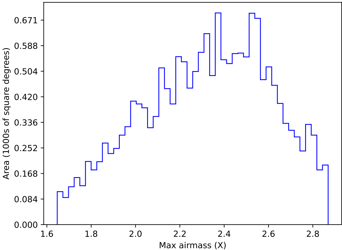
too_elab_r32_d2_ugrizy_v3.4_10yrs WFD y band: Max airmass
