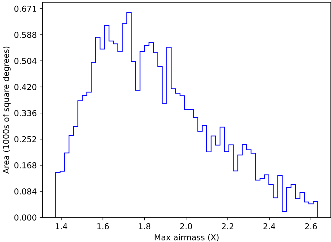
too_elab_r32_d2_ugrizy_v3.4_10yrs WFD u band: Max airmass
