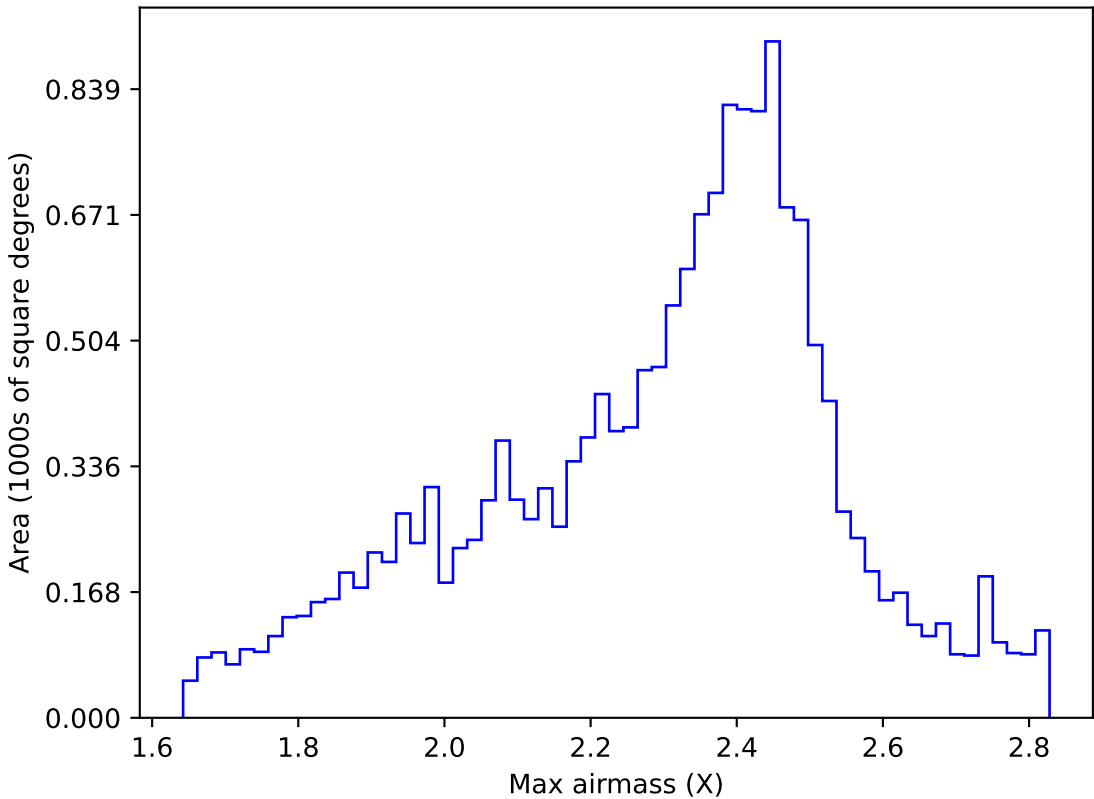
too_elab_r32_d2_ugrizy_v3.4_10yrs WFD r band: Max airmass
