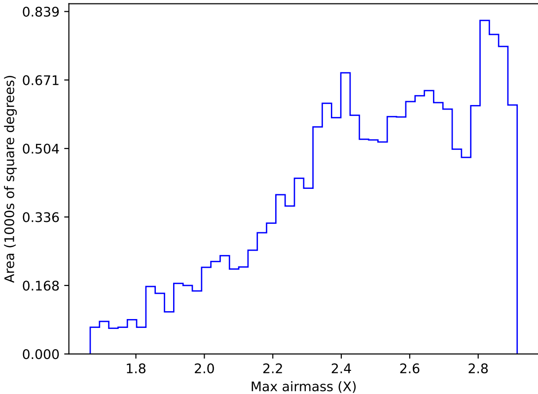
too_elab_r32_d2_ugrizy_v3.4_10yrs WFD i band: Max airmass
