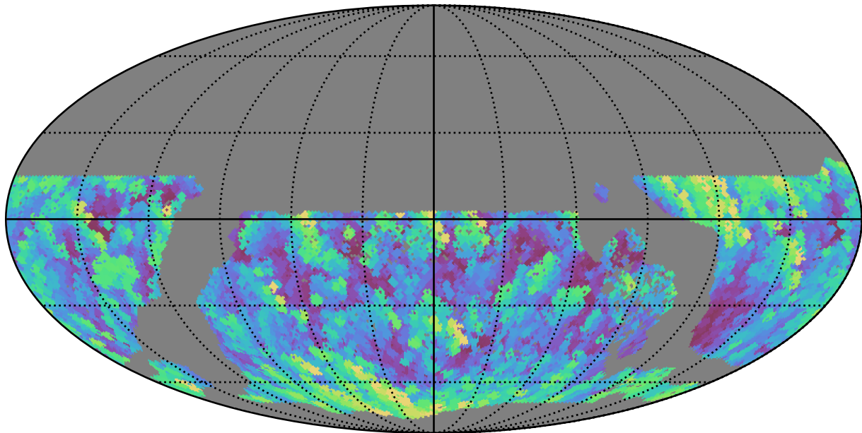
too_elab_r32_d2_ugrizy_v3.4_10yrs WFD g band: Max airmass
