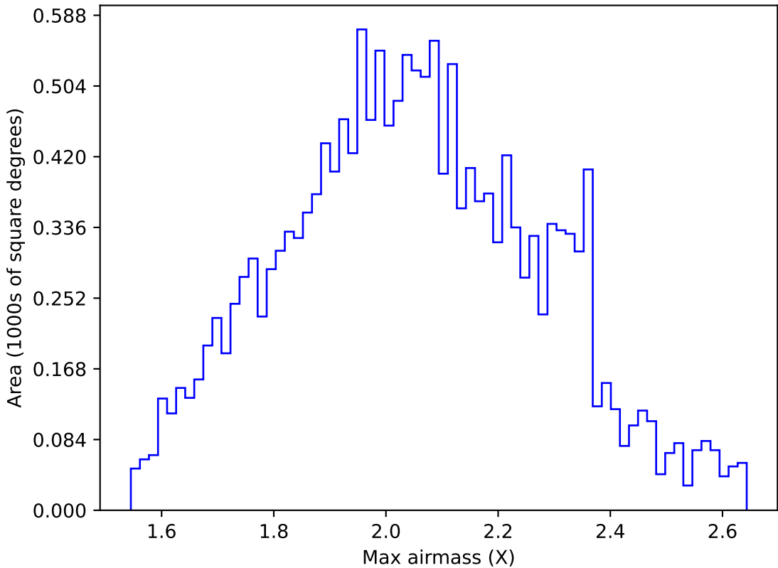
too_elab_r32_d2_ugrizy_v3.4_10yrs WFD g band: Max airmass
