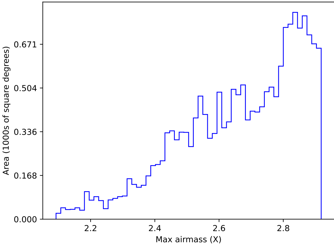
too_elab_r32_d2_ugrizy_v3.4_10yrs WFD all bands: Max airmass
