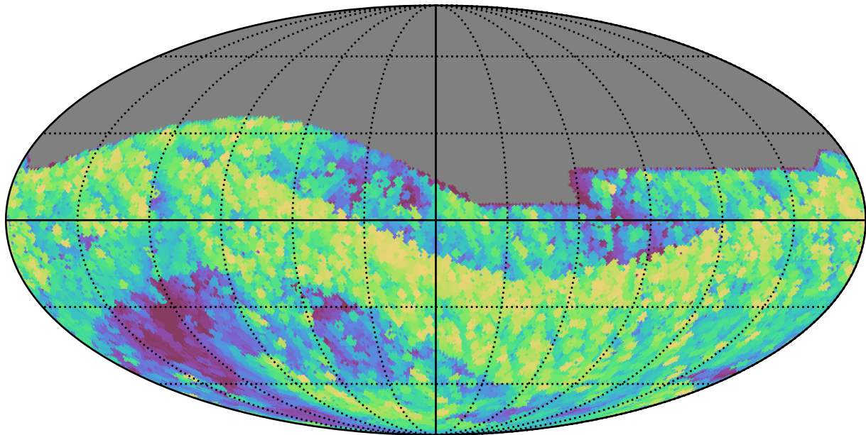
too_elab_r32_d2_ugrizy_v3.4_10yrs All sky z band: Max airmass
