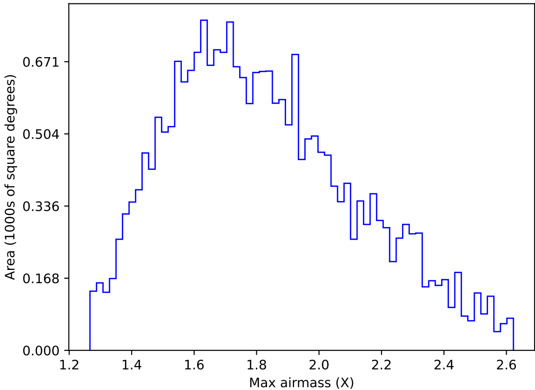
too_elab_r32_d2_ugrizy_v3.4_10yrs All sky u band: Max airmass
