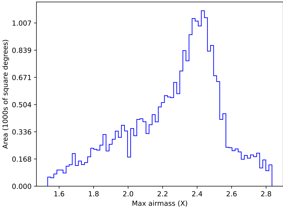
too_elab_r32_d2_ugrizy_v3.4_10yrs All sky r band: Max airmass
