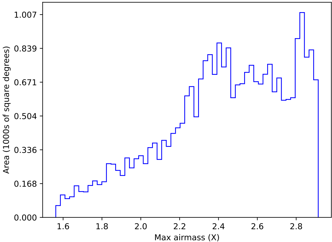
too_elab_r32_d2_ugrizy_v3.4_10yrs All sky i band: Max airmass
