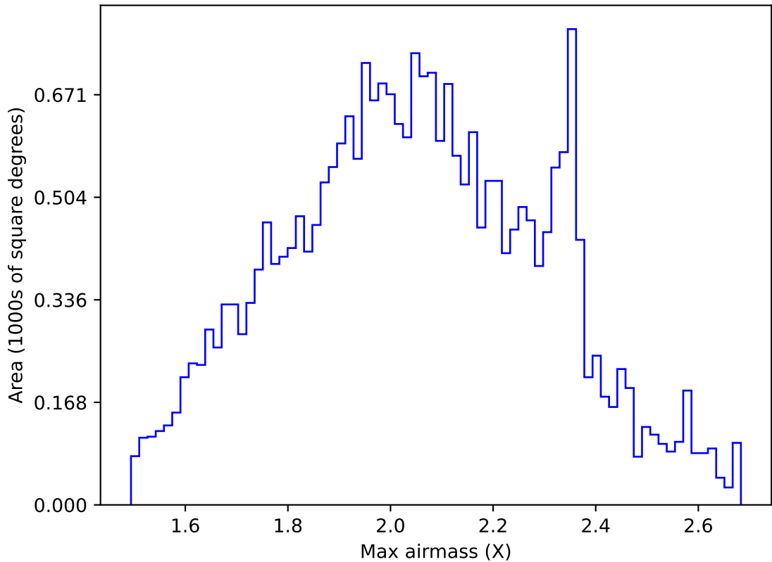
too_elab_r32_d2_ugrizy_v3.4_10yrs All sky g band: Max airmass
