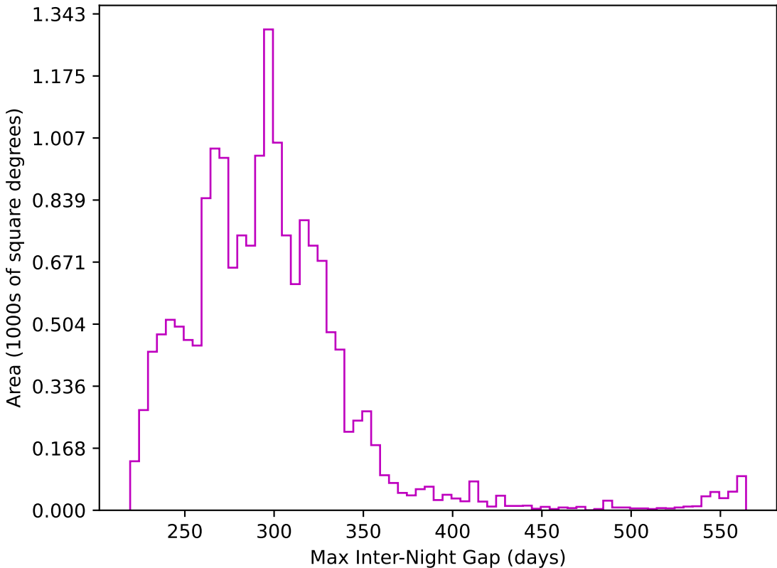
too_elab_r32_d2_ugrizyv3.4_10yrs WFD z band: Max Inter-Night Gap
