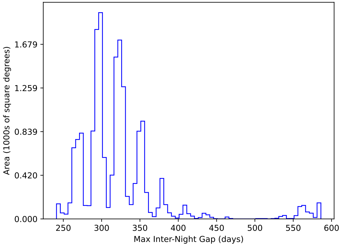
too_elab_r32_d2_ugrizyv3.4_10yrs WFD y band: Max Inter-Night Gap
