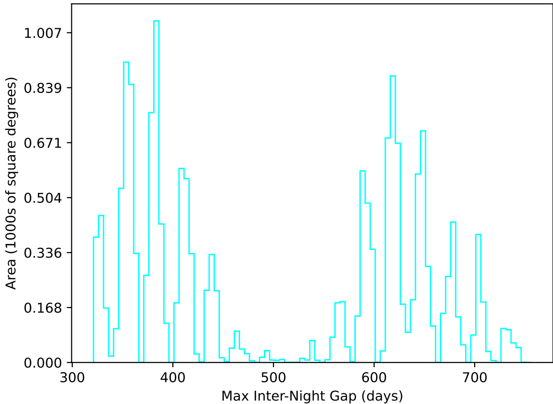
too_elab_r32_d2_ugrizyv3.4_10yrs WFD u band: Max Inter-Night Gap
