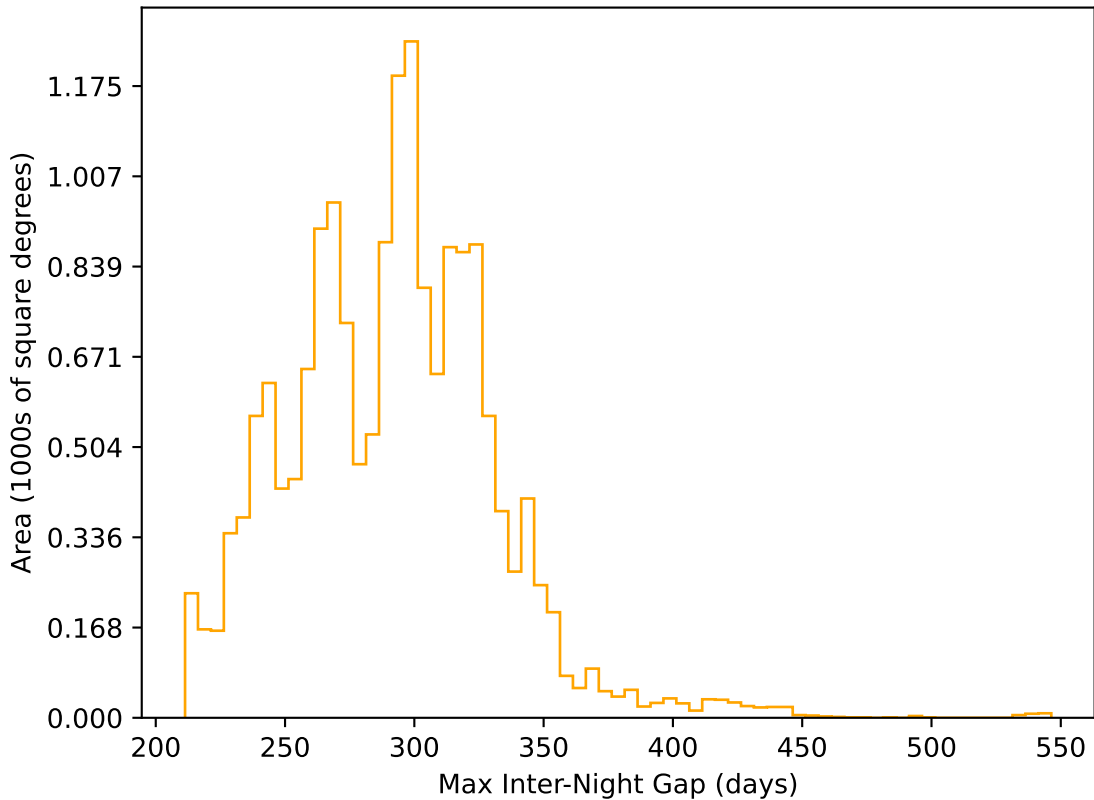
too_elab_r32_d2_ugrizy_v3.4_10yrs WFD r band: Max Inter-Night Gap
