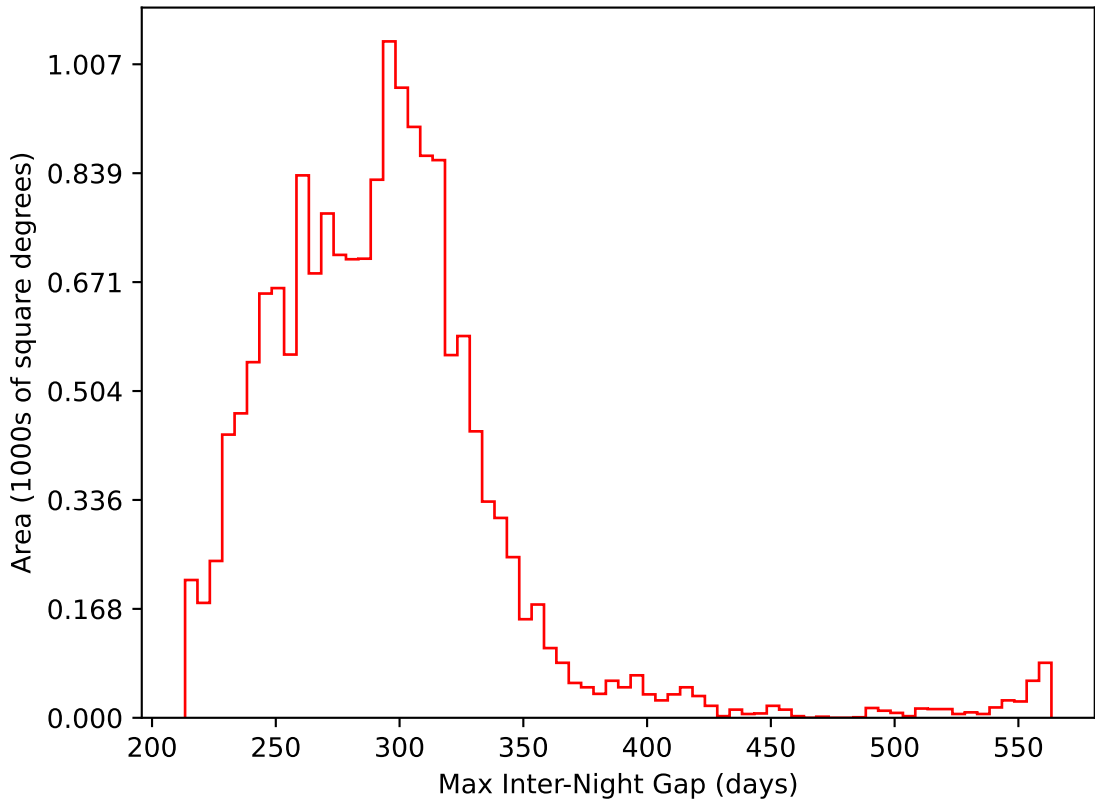
too_elab_r32_d2_ugrizy_v3.4_10yrs WFD i band: Max Inter-Night Gap
