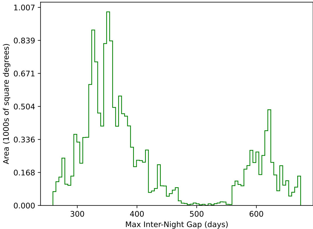
too_elab_r32_d2_ugrizyv3.4_10yrs WFD g band: Max Inter-Night Gap
