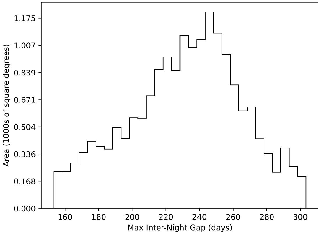
too_elab_r32_d2_ugrizy_v3.4_10yrs WFD all bands: Max Inter-Night Gap
