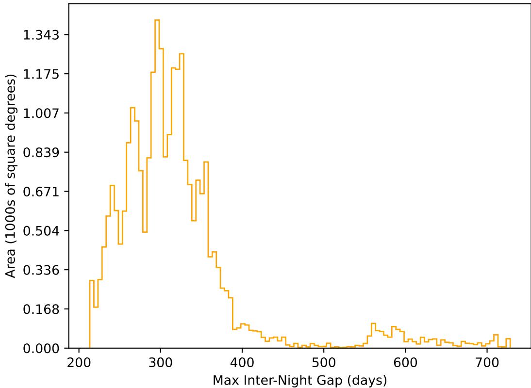
too_elab_r32_d2_ugrizy_v3.4_10yrs All sky r band: Max Inter-Night Gap
