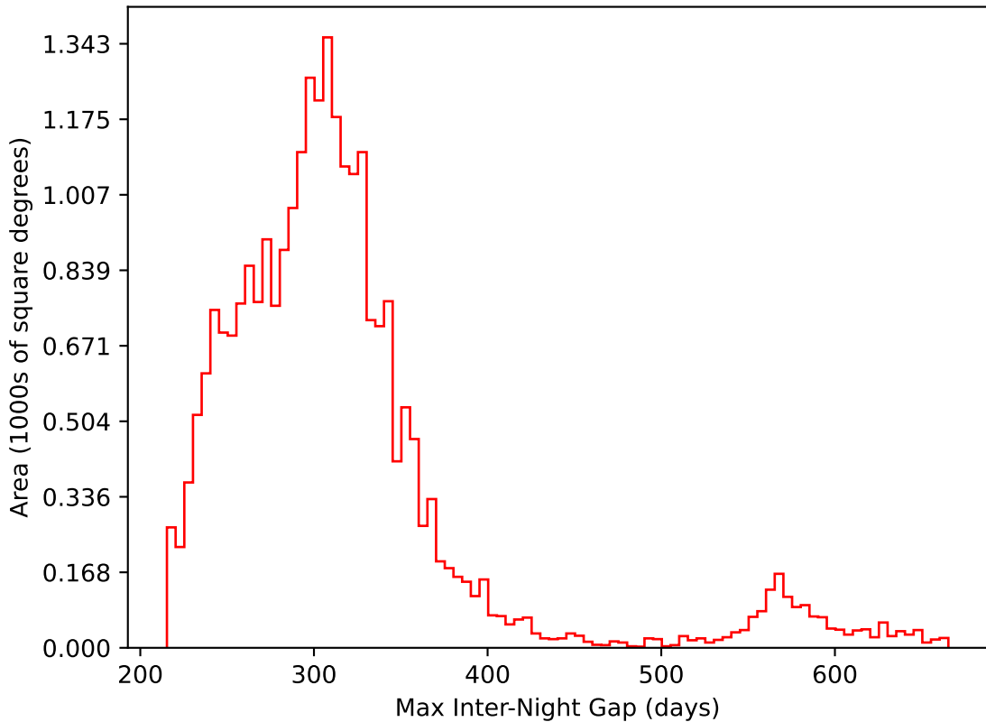
too_elab_r32_d2_ugrizy_v3.4_10yrs All sky i band: Max Inter-Night Gap
