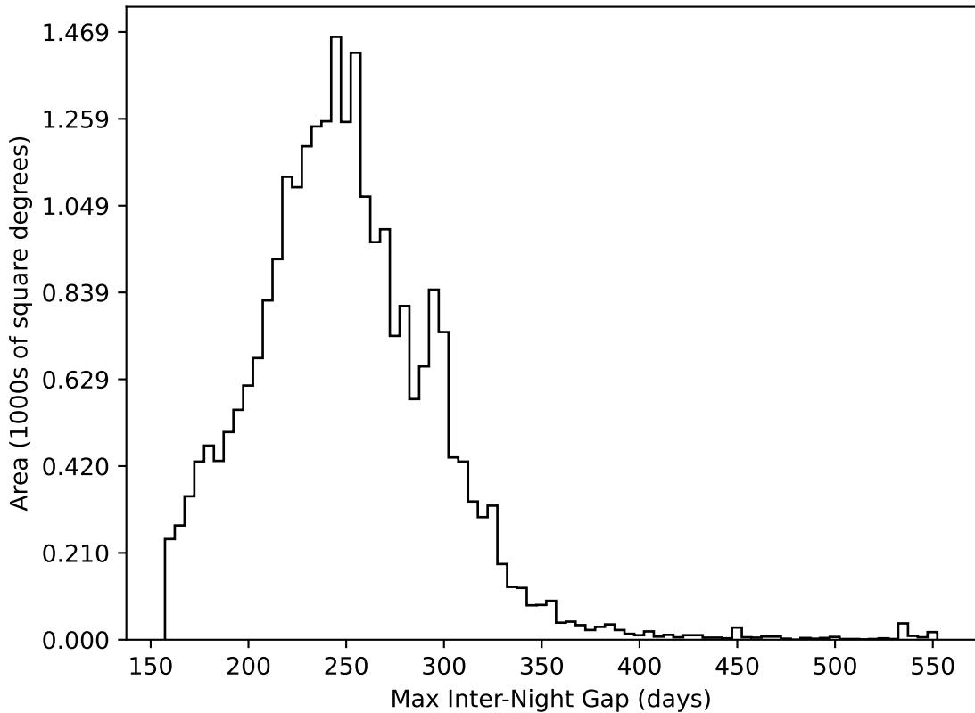
too_elab_r32_d2_ugrizy_v3.4_10yrs All sky all bands: Max Inter-Night Gap
