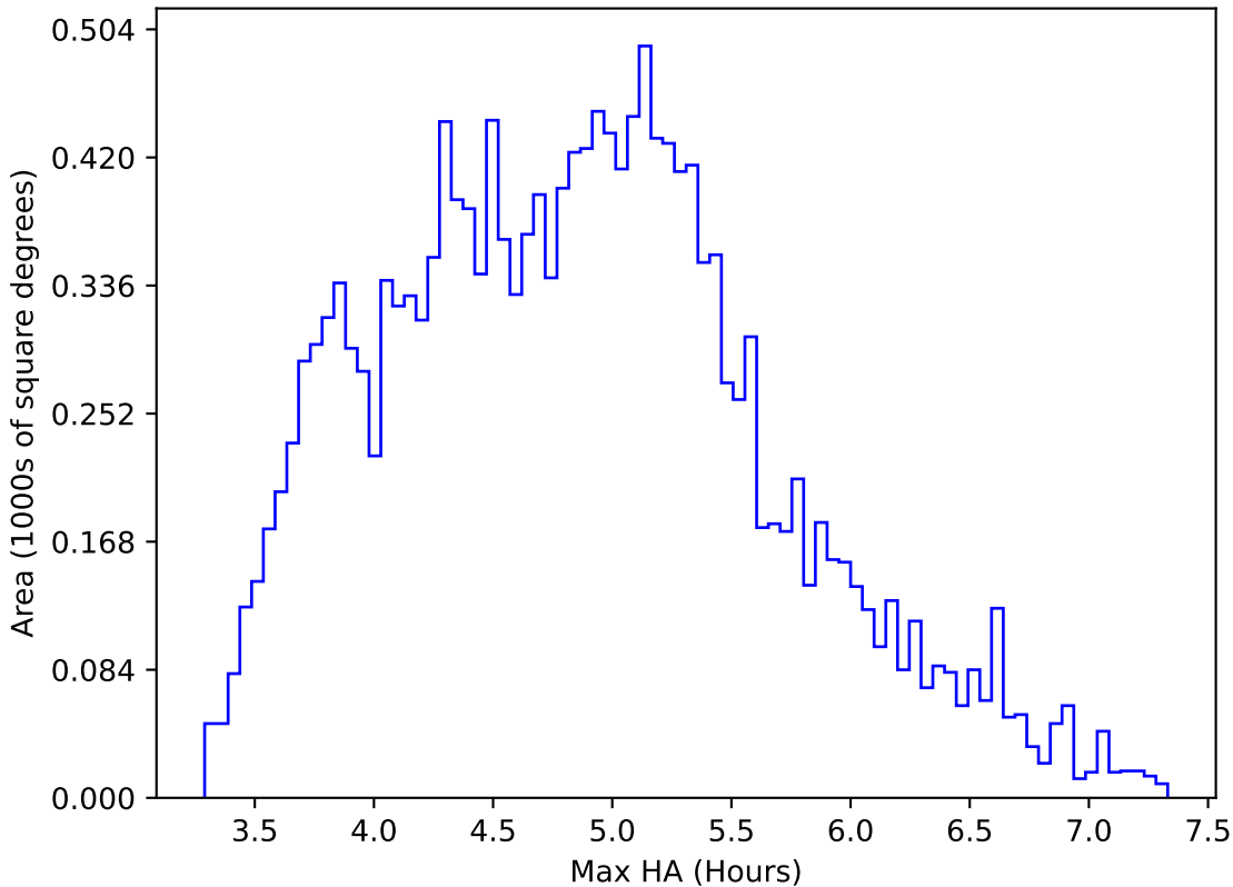
too_elab_r32_d2_ugrizy_v3.4_10yrs WFD z band: Max HA
