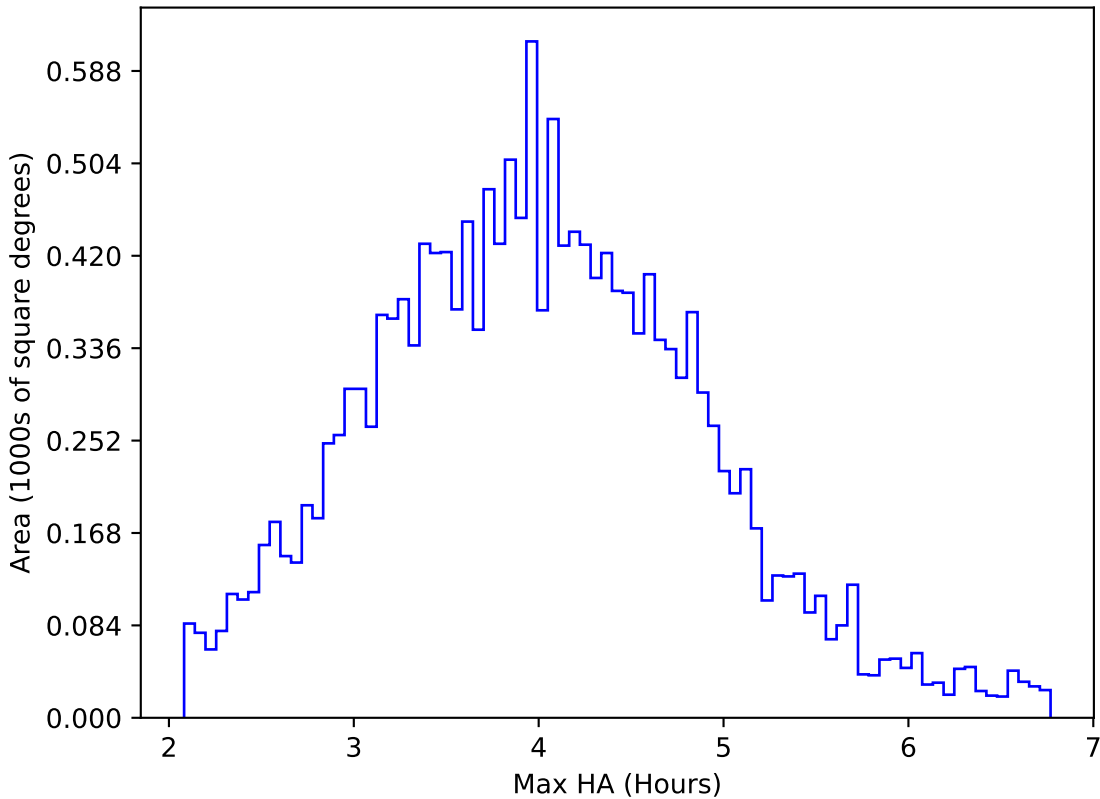
too_elab_r32_d2_ugrizy_v3.4_10yrs WFD u band: Max HA
