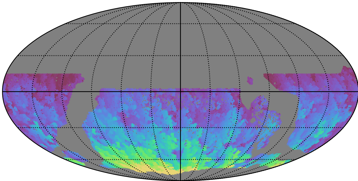
too_elab_r32_d2_ugrizy_v3.4_10yrs WFD r band: Max HA
