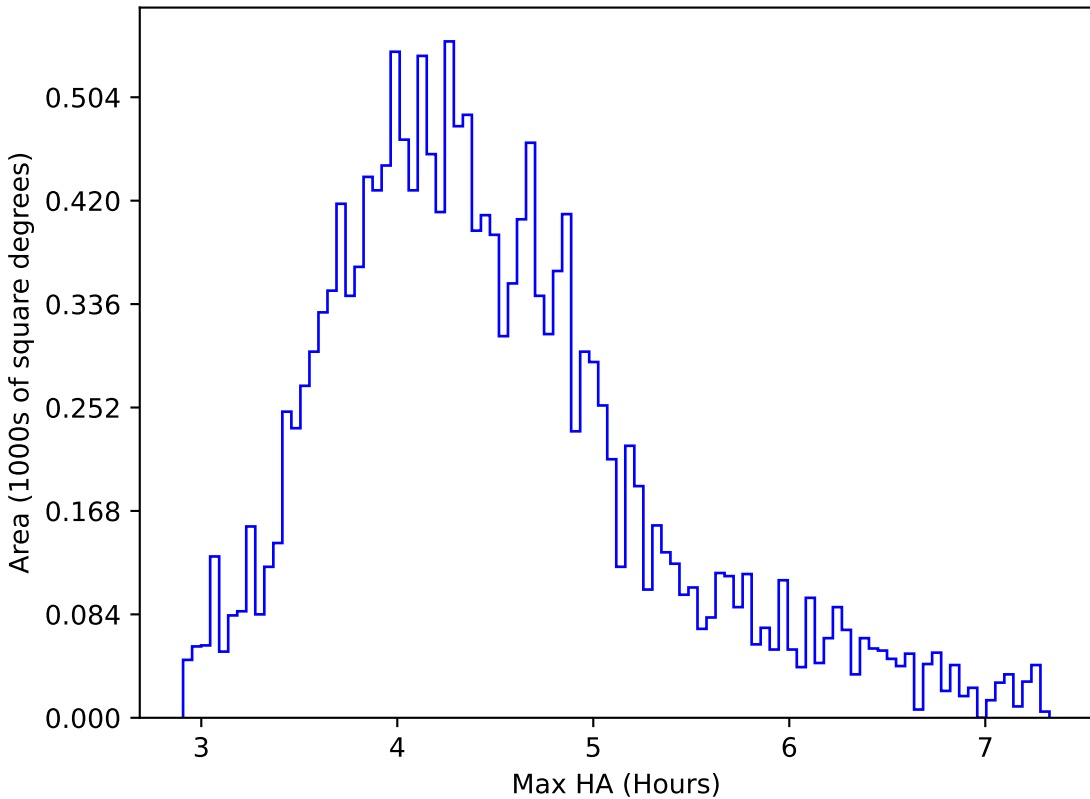
too_elab_r32_d2_ugrizy_v3.4_10yrs WFD r band: Max HA
