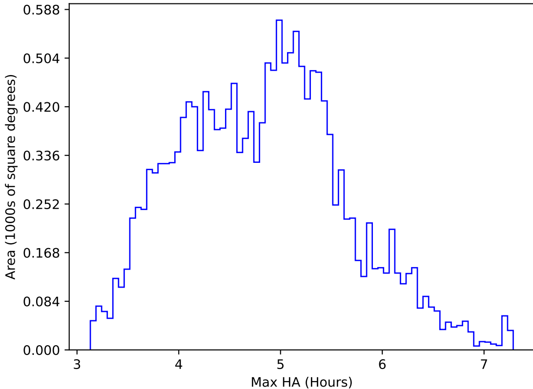
too_elab_r32_d2_ugrizy_v3.4_10yrs WFD i band: Max HA
