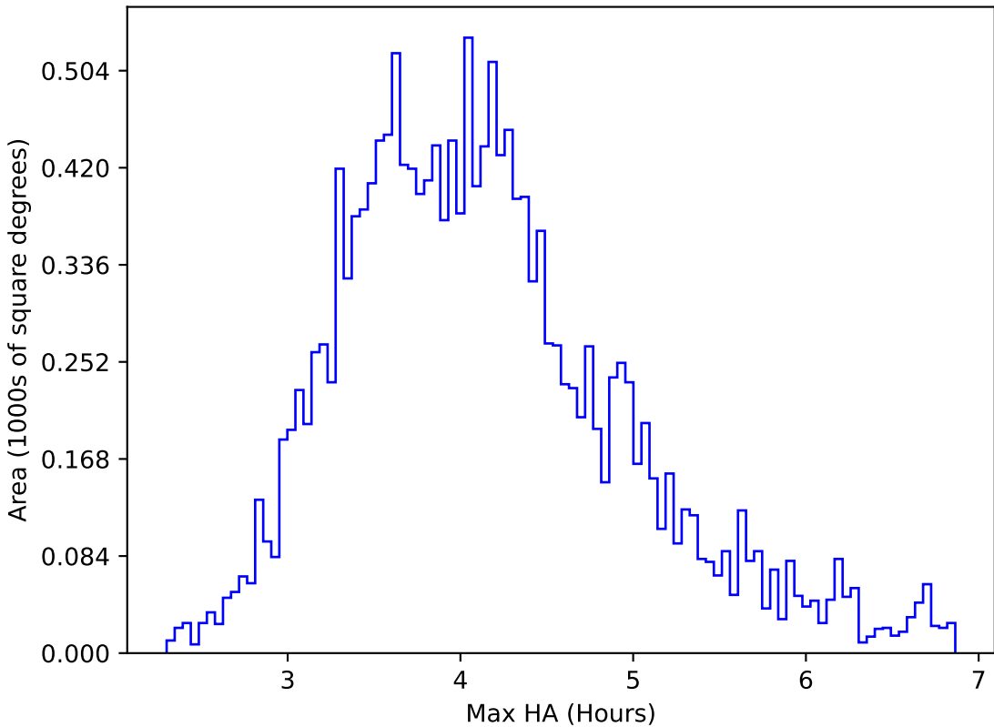
too_elab_r32_d2_ugrizy_v3.4_10yrs WFD g band: Max HA
