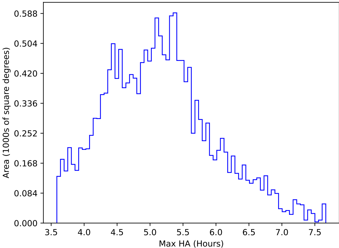
too_elab_r32_d2_ugrizy_v3.4_10yrs WFD all bands: Max HA
