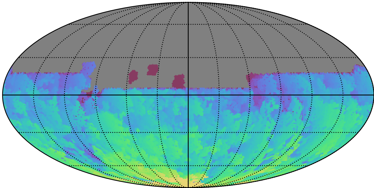
too_elab_r32_d2_ugrizy_v3.4_10yrs All sky u band: Max HA
