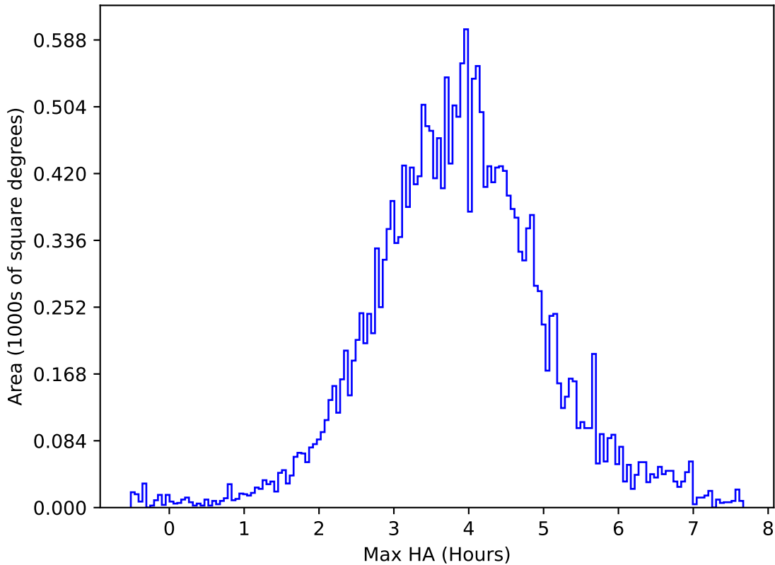
too_elab_r32_d2_ugrizy_v3.4_10yrs All sky u band: Max HA
