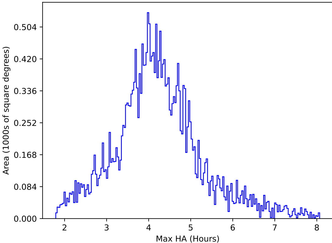
too_elab_r32_d2_ugrizy_v3.4_10yrs All sky r band: Max HA
