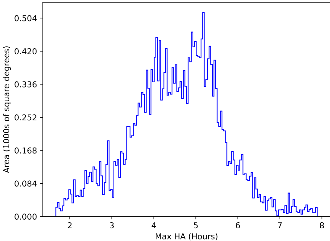
too_elab_r32_d2_ugrizy_v3.4_10yrs All sky i band: Max HA
