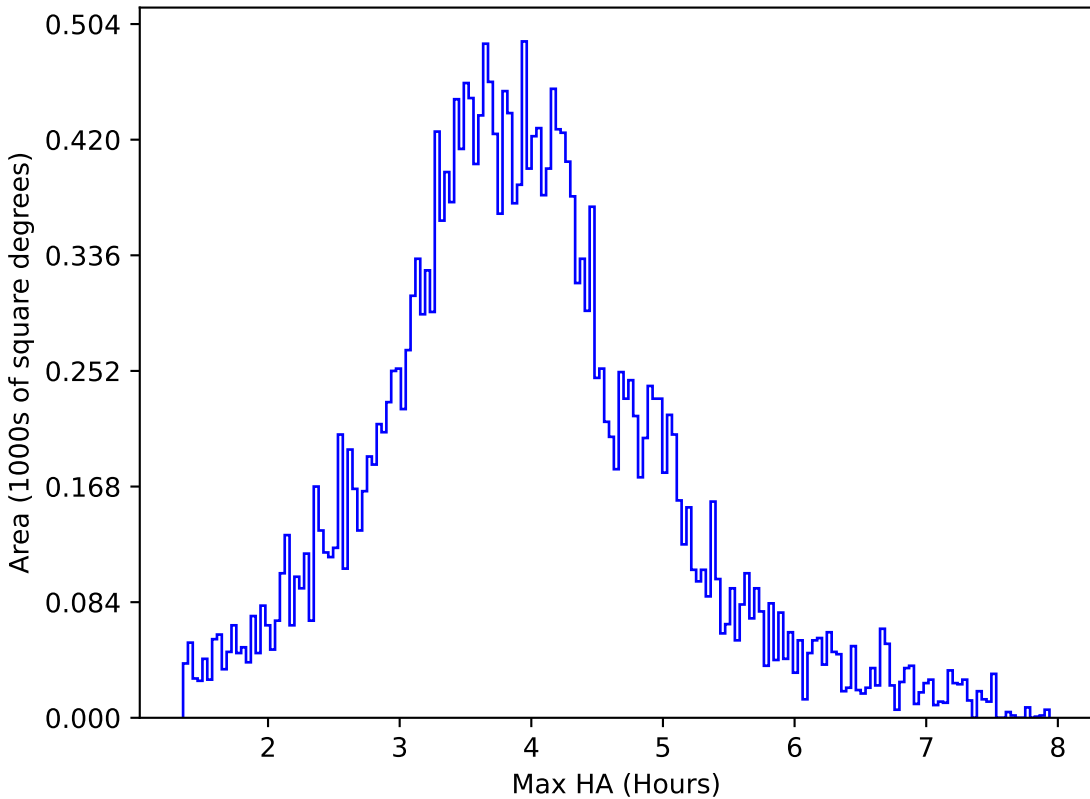
too_elab_r32_d2_ugrizy_v3.4_10yrs All sky g band: Max HA
