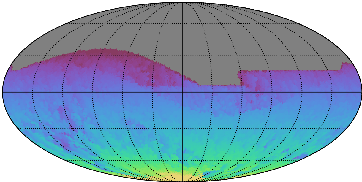
too_elab_r32_d2_ugrizy_v3.4_10yrs All sky all bands: Max HA
