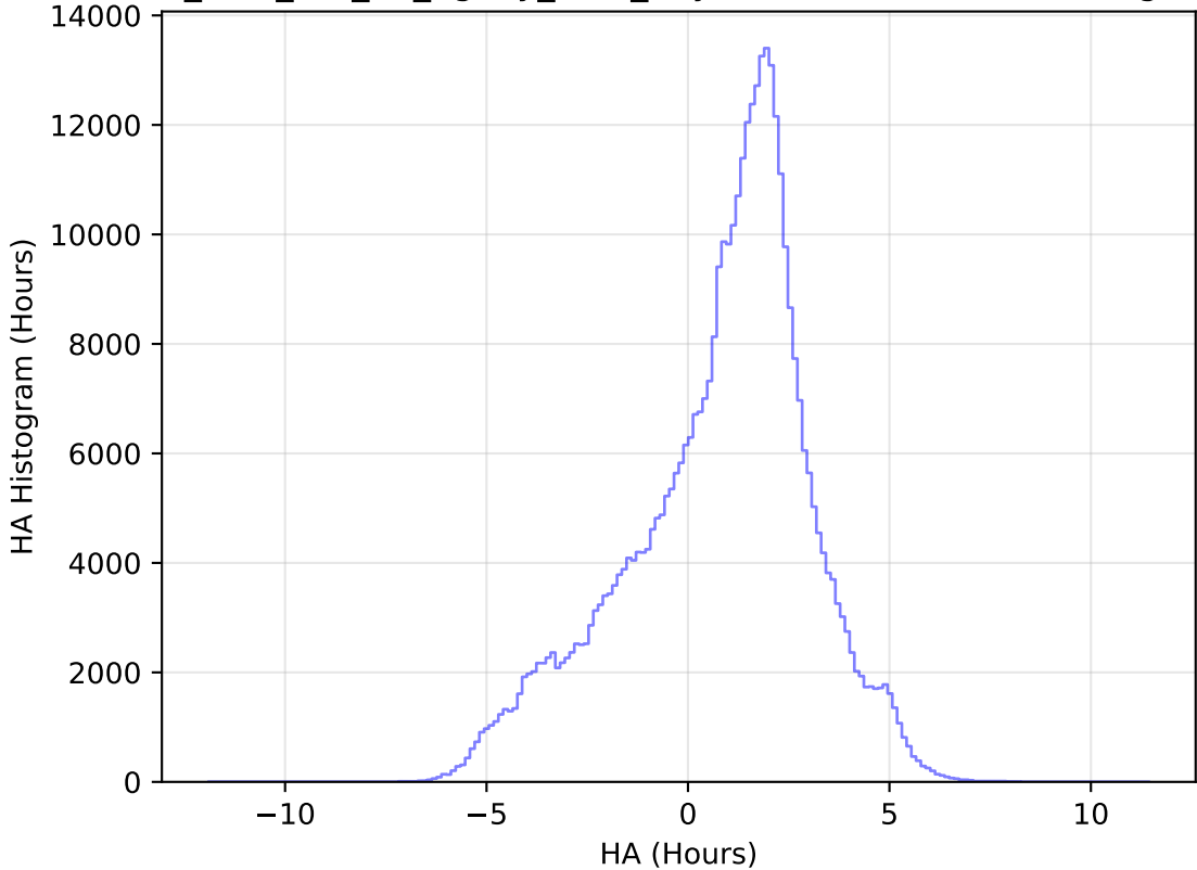
too_elab_r32_d2_ugrizy_v3.4_10yrs WFD z band: HA Histogram
