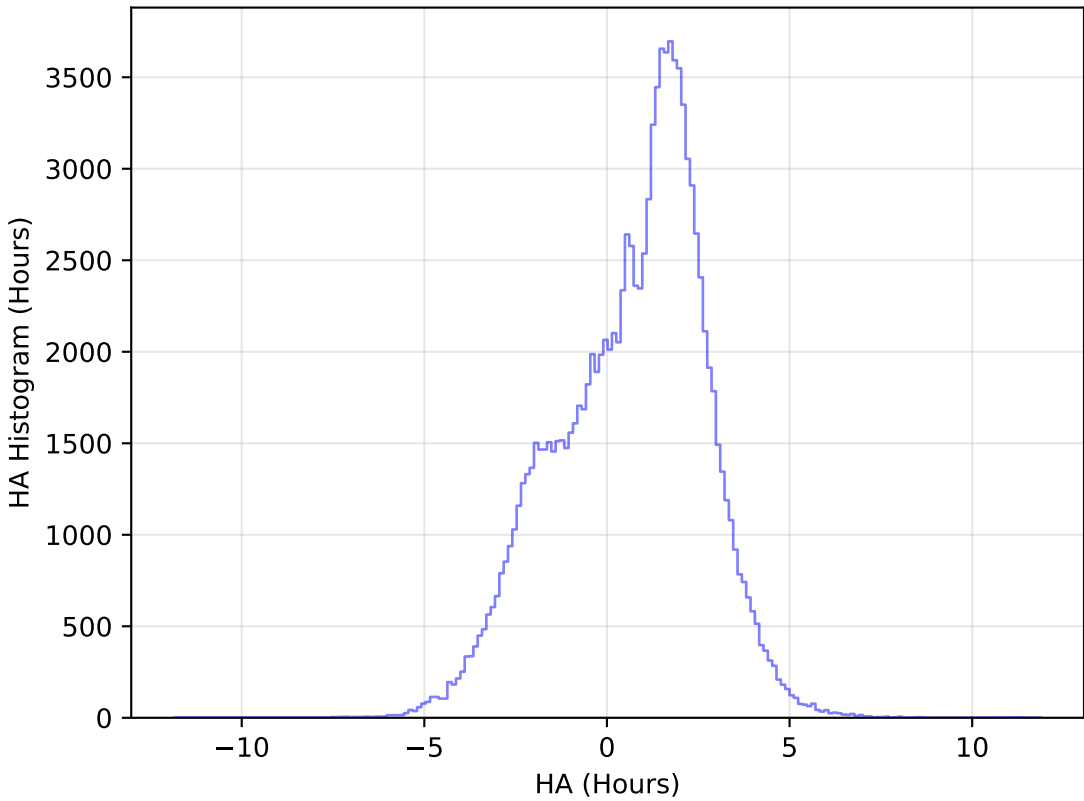
too_elab_r32_d2_ugrizy_v3.4_10yrs WFD u band: HA Histogram
