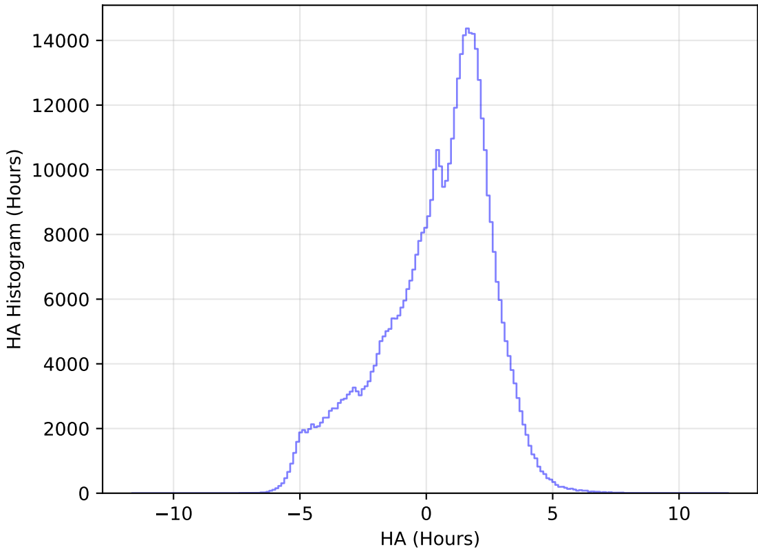
too_elab_r32_d2_ugrizy_v3.4_10yrs WFD r band: HA Histogram
