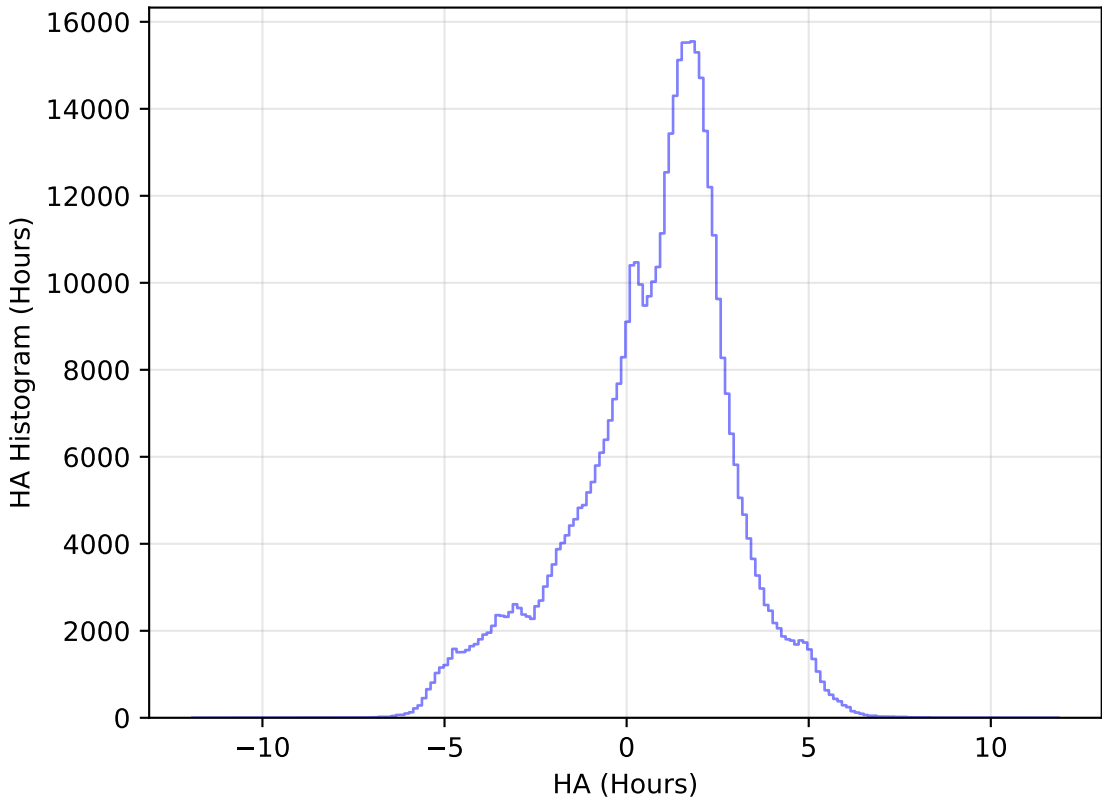
too_elab_r32_d2_ugrizy_v3.4_10yrs WFD i band: HA Histogram
