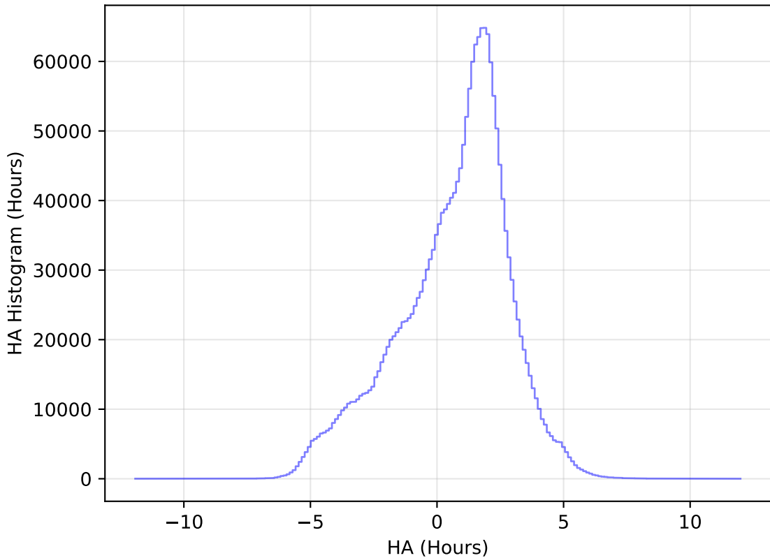
too_elab_r32_d2_ugrizy_v3.4_10yrs WFD all bands: HA Histogram
