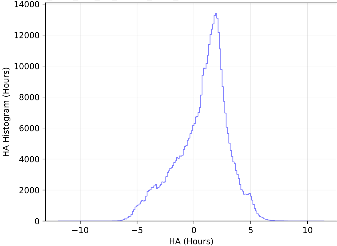
too_elab_r32_d2_ugrizy_v3.4_10yrs All sky z band: HA Histogram
