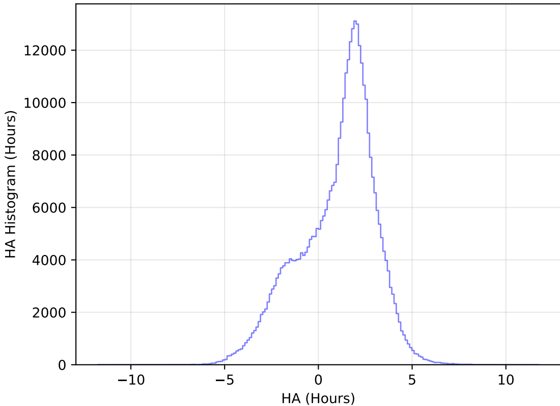
too_elab_r32_d2_ugrizy_v3.4_10yrs All sky y band: HA Histogram
