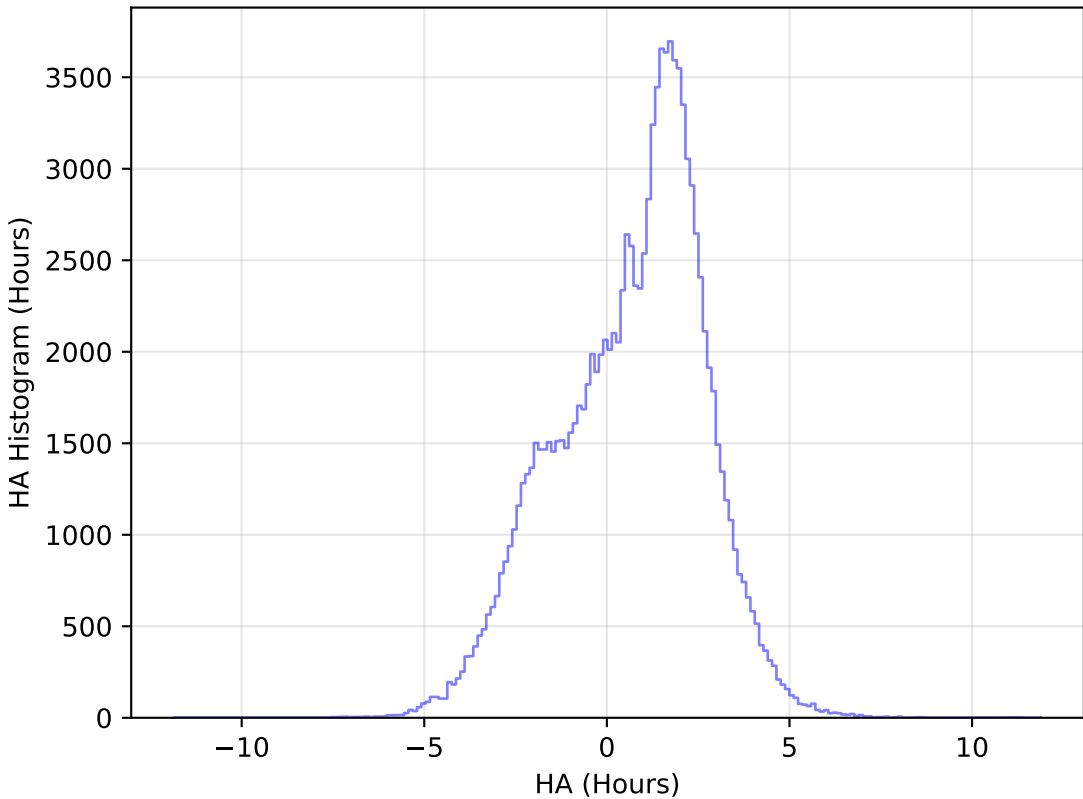
too_elab_r32_d2_ugrizy_v3.4_10yrs All sky u band: HA Histogram
