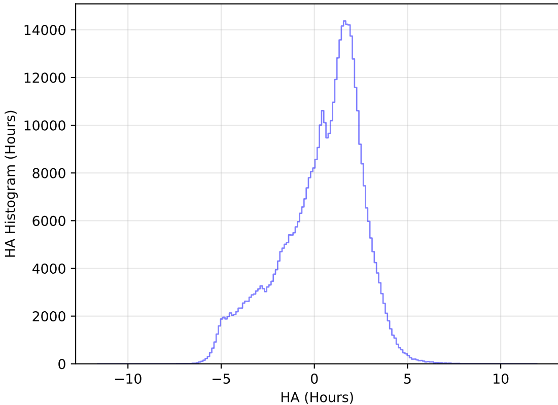
too_elab_r32_d2_ugrizy_v3.4_10yrs All sky r band: HA Histogram
